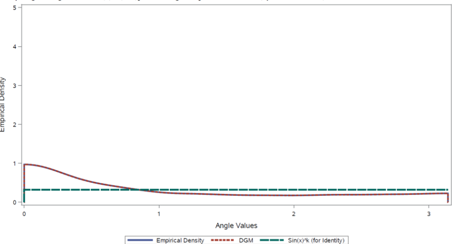
Emp Angles-targ Dists v \sin(x)^k(k=1) [row=5, Angle#=1]: DGM=MVTVNS (epan-SILVR09-15), Mat=5x5, #Obs=6, #Sims = 10000
