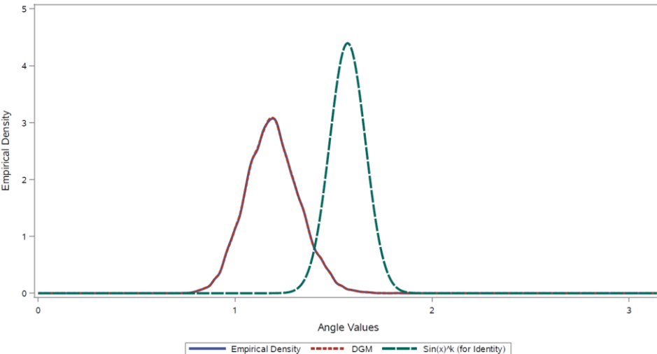
Emp Angles-targ Dists v \text{Sin}(x)^k(k=2) [row=4, Angle#=2]: DGM=MVTVNS (epan-SILVR09-15), Mat=5x5, #Obs=126, #Sims = 10000
