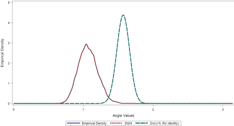
Emp Angles-targ Dists v \sin(x)^k(k=1) [row=5, Angle#=1]: DGM=MVTVNS (epan-SILVR09-15), Mat=5x5, #Obs=126, #Sims = 10000
