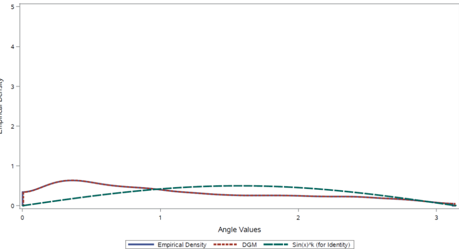
Emp Angles-targ Dists v \text{Sin}(x)^k(k=2) [row=4, Angle#=2]: DGM=MVTVNS (epan-SILVR09-15), Mat=5x5, #Obs=6, #Sims = 10000
